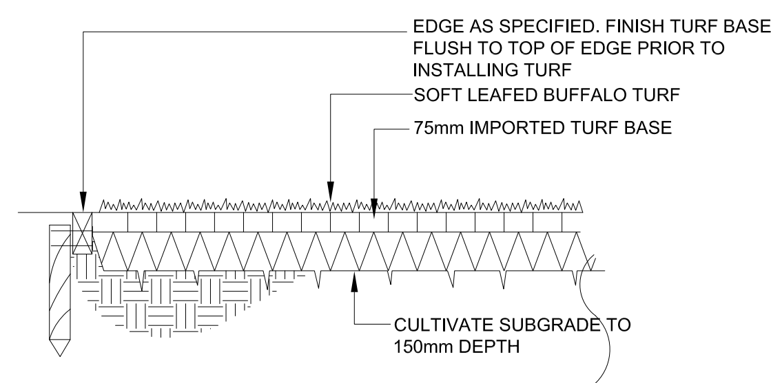
3 TURF ON GRADE TYPICAL SECTION 1:20
